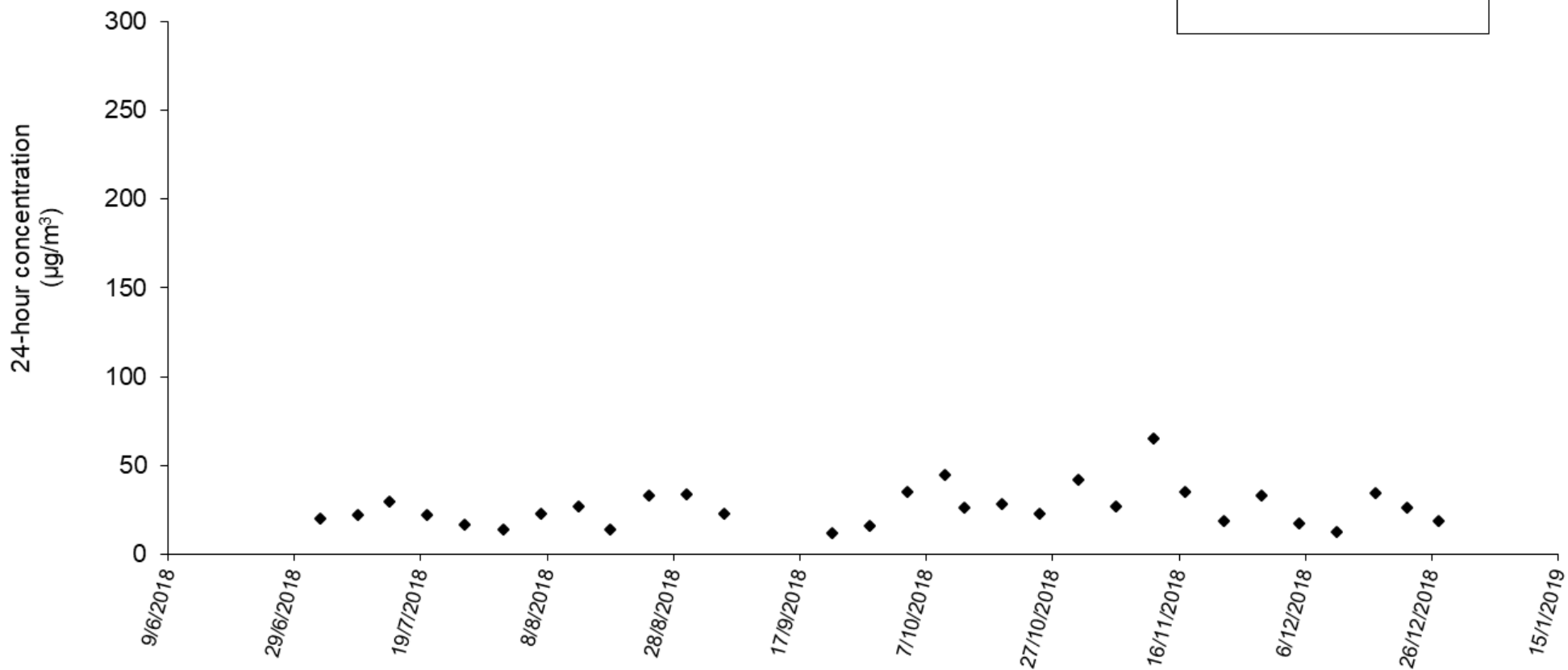
24-hour TSP concentration vs date for Location M-A3
